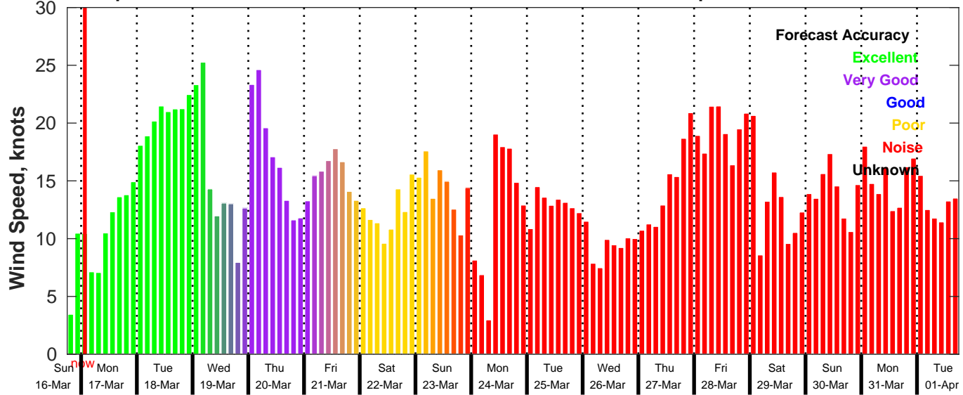
GFS Wind Speed Forecast for NDBC 42019 from 16-Mar-2025 18:00:00 to 01-Apr-2025 18:00:00
