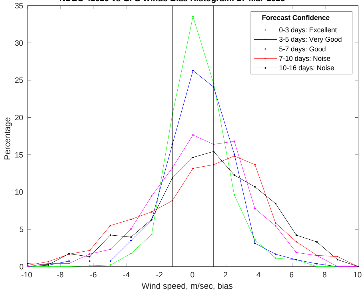
NDBC 42020 vs GFS Winds Bias Histogram: 17-Mar-2025
