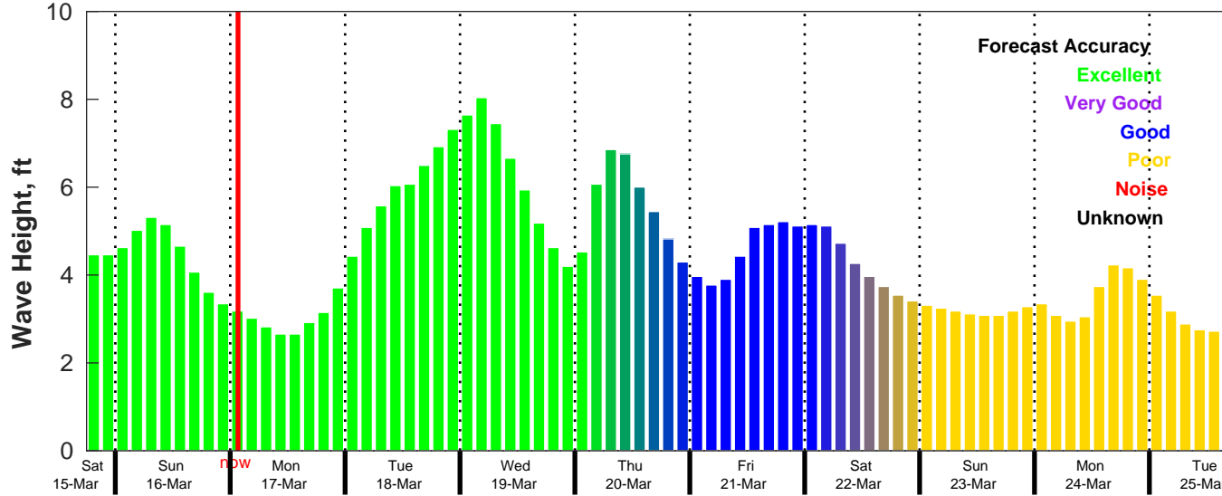
CMEMS Wave Forecast for NDBC 42020 from 15-Mar-2025 18:00:00 to 25-Mar-2025 18:00:00
