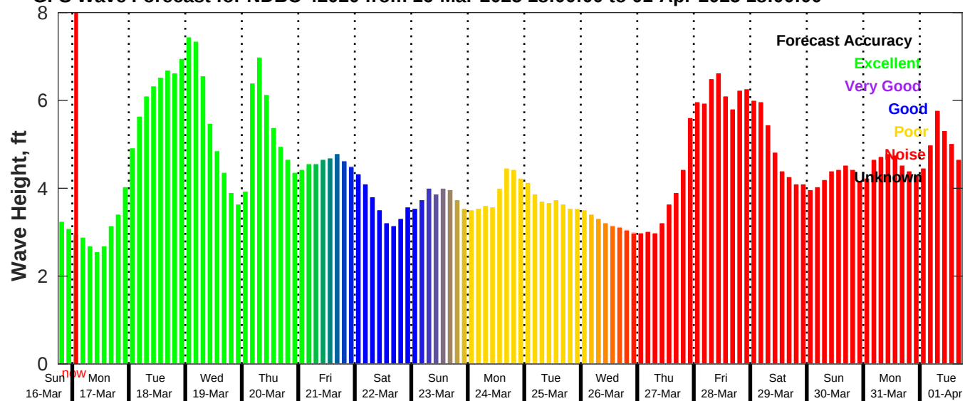
GFS Wave Forecast for NDBC 42020 from 16-Mar-2025 18:00:00 to 01-Apr-2025 18:00:00
