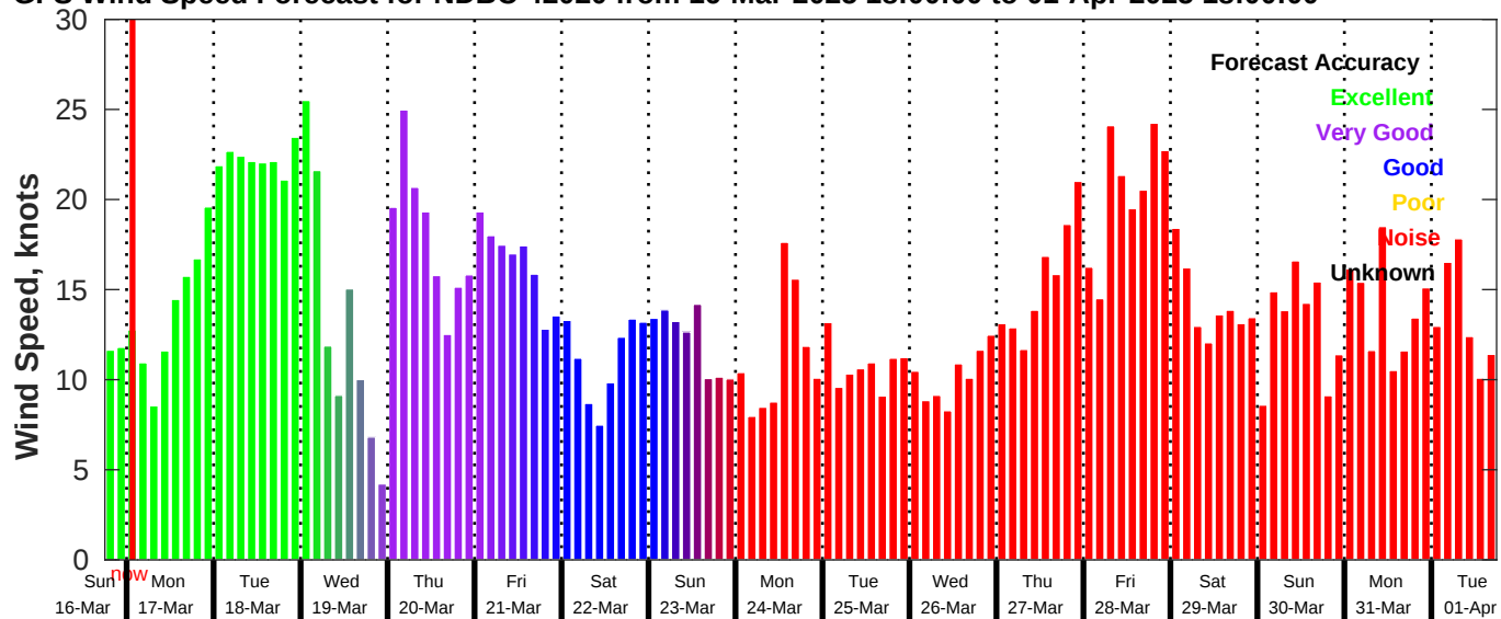
GFS Wind Speed Forecast for NDBC 42020 from 16-Mar-2025 18:00:00 to 01-Apr-2025 18:00:00
