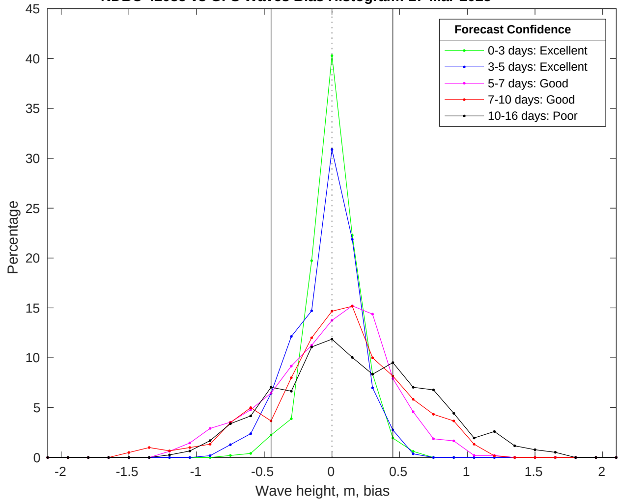
NDBC 42035 vs GFS Waves Bias Histogram: 17-Mar-2025
