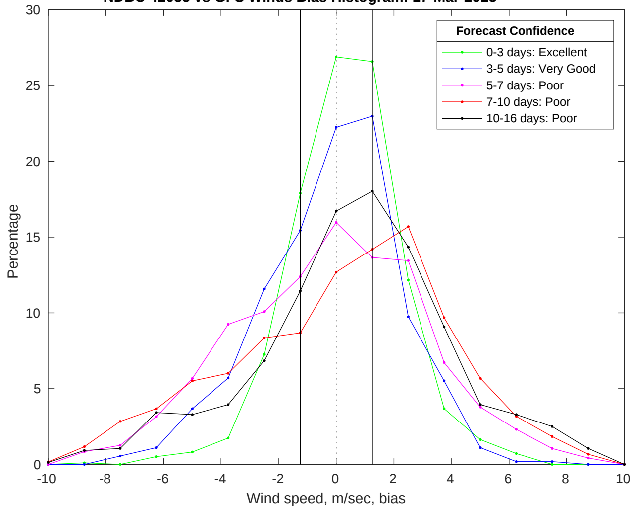
NDBC 42035 vs GFS Winds Bias Histogram: 17-Mar-2025
