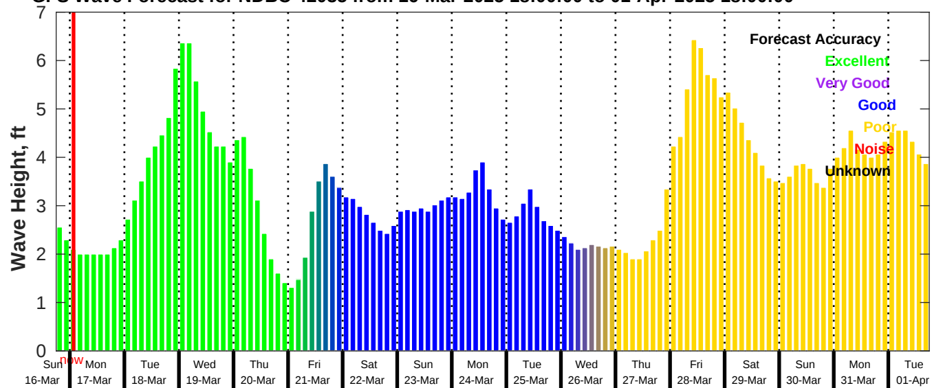
GFS Wave Forecast for NDBC 42035 from 16-Mar-2025 18:00:00 to 01-Apr-2025 18:00:00
