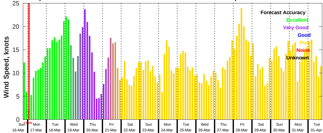
GFS Wind Speed Forecast for NDBC 42035 from 16-Mar-2025 18:00:00 to 01-Apr-2025 18:00:00
