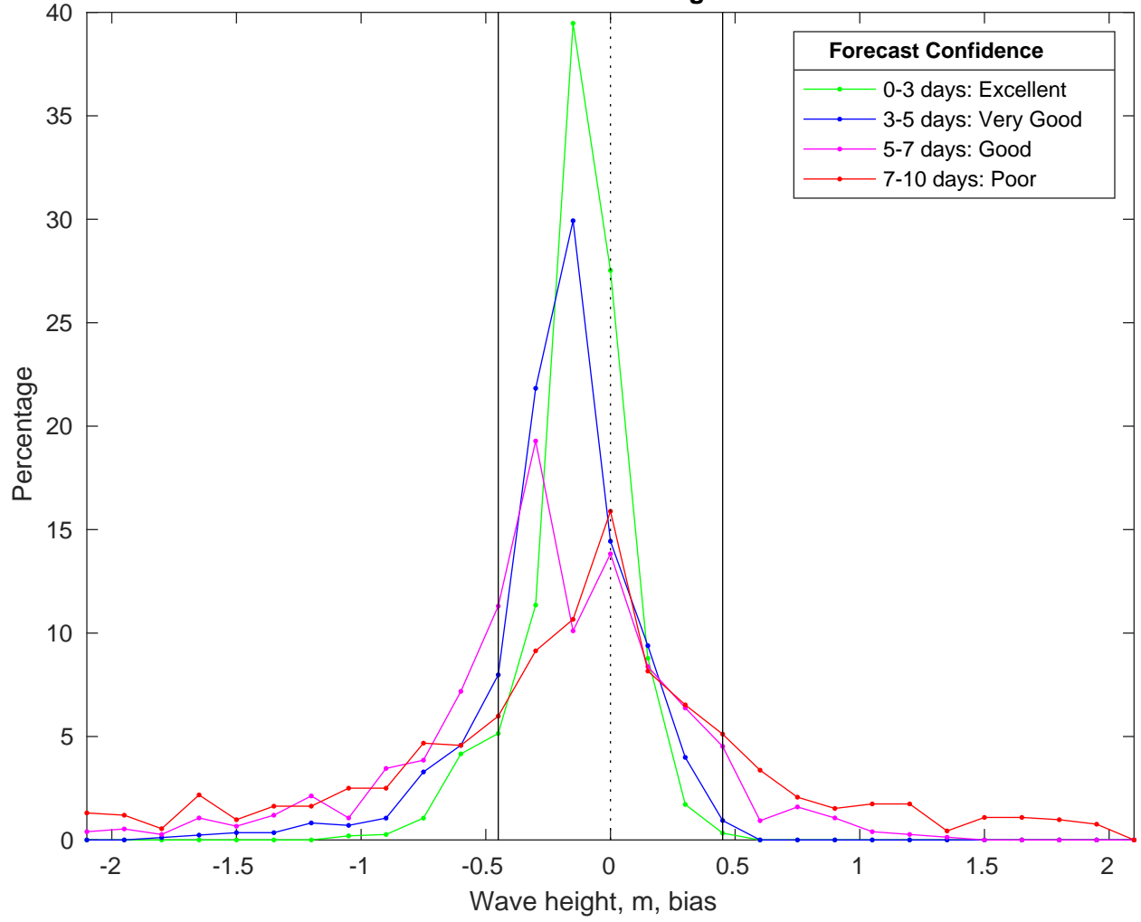
NDBC 42036 vs CMEMS Waves Bias Histogram: 17-Mar-2025
