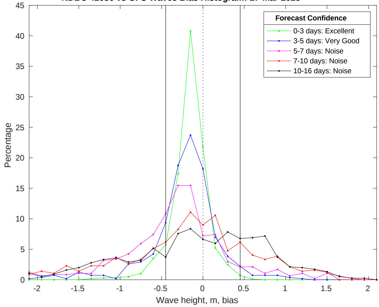
NDBC 42036 vs GFS Waves Bias Histogram: 17-Mar-2025
