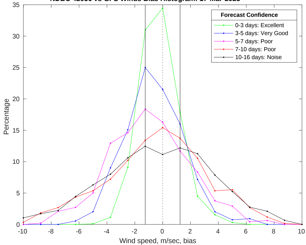
NDBC 42036 vs GFS Winds Bias Histogram: 17-Mar-2025
