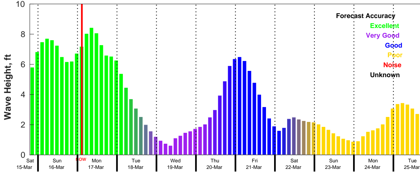
CMEMS Wave Forecast for NDBC 42036 from 15-Mar-2025 19:00:00 to 25-Mar-2025 19:00:00
