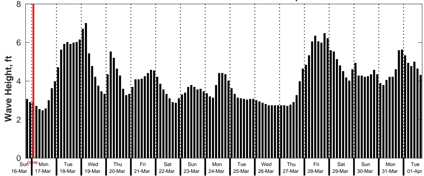
GFS Wave Forecast for NDBC 42092 from 16-Mar-2025 18:00:00 to 01-Apr-2025 18:00:00
