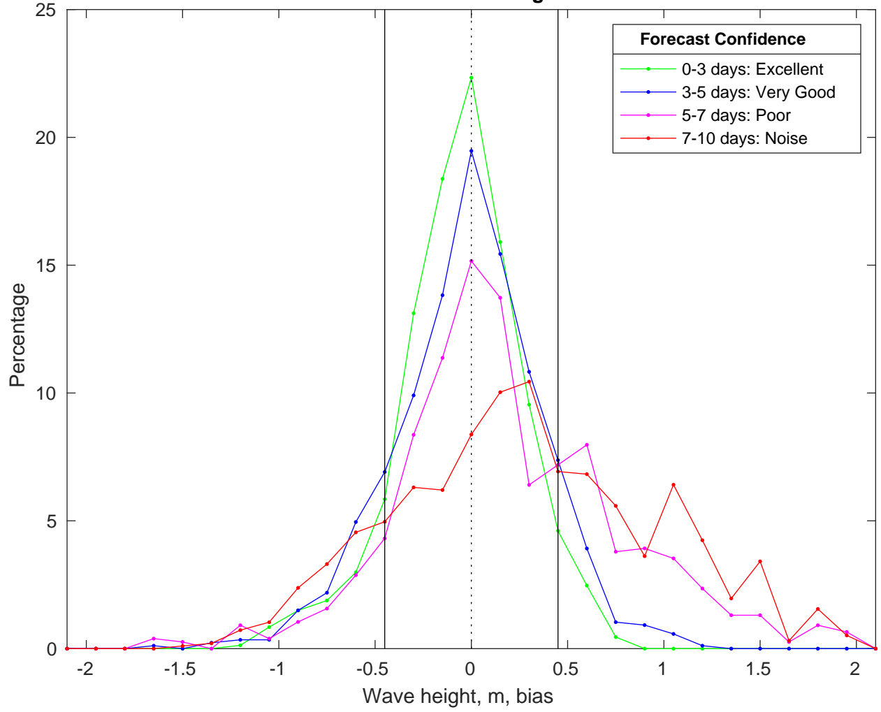
NDBC 46011 vs CMEMS Waves Bias Histogram: 17-Mar-2025
