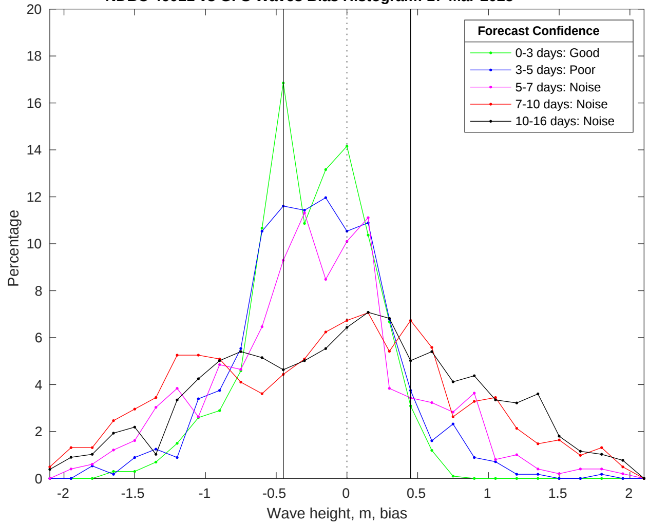
NDBC 46011 vs GFS Waves Bias Histogram: 17-Mar-2025
