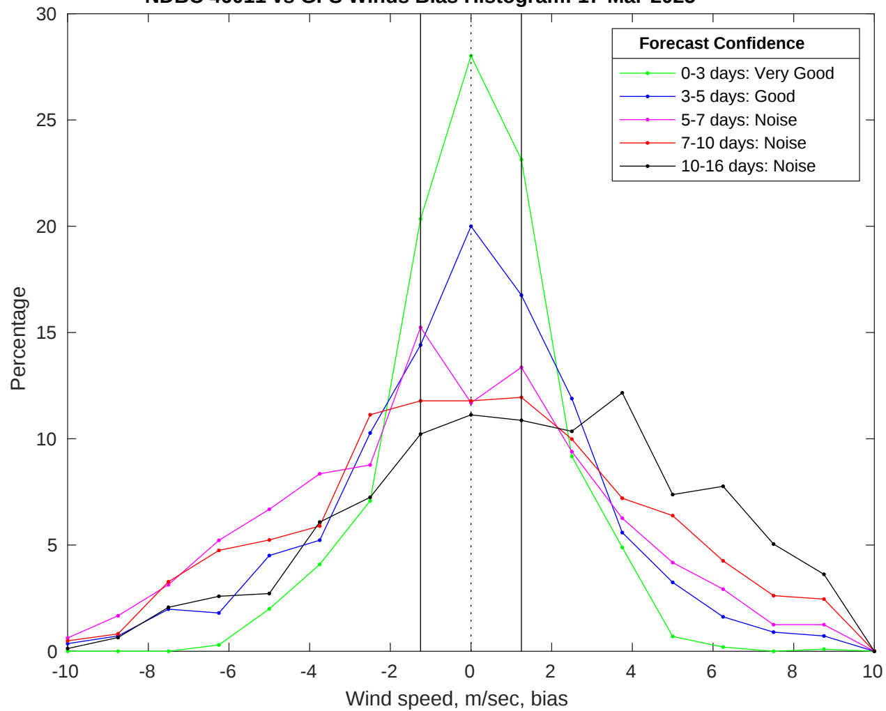
NDBC 46011 vs GFS Winds Bias Histogram: 17-Mar-2025
