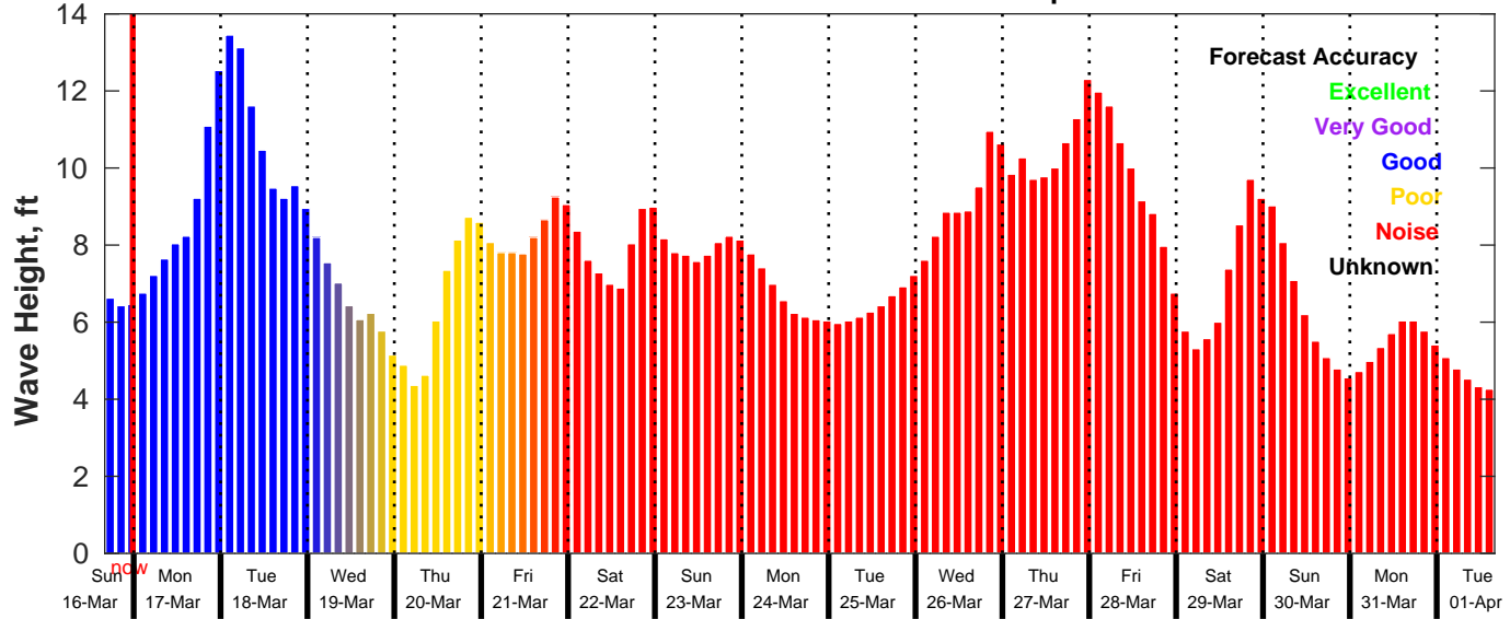
GFS Wave Forecast for NDBC 46011 from 16-Mar-2025 16:00:00 to 01-Apr-2025 16:00:00
