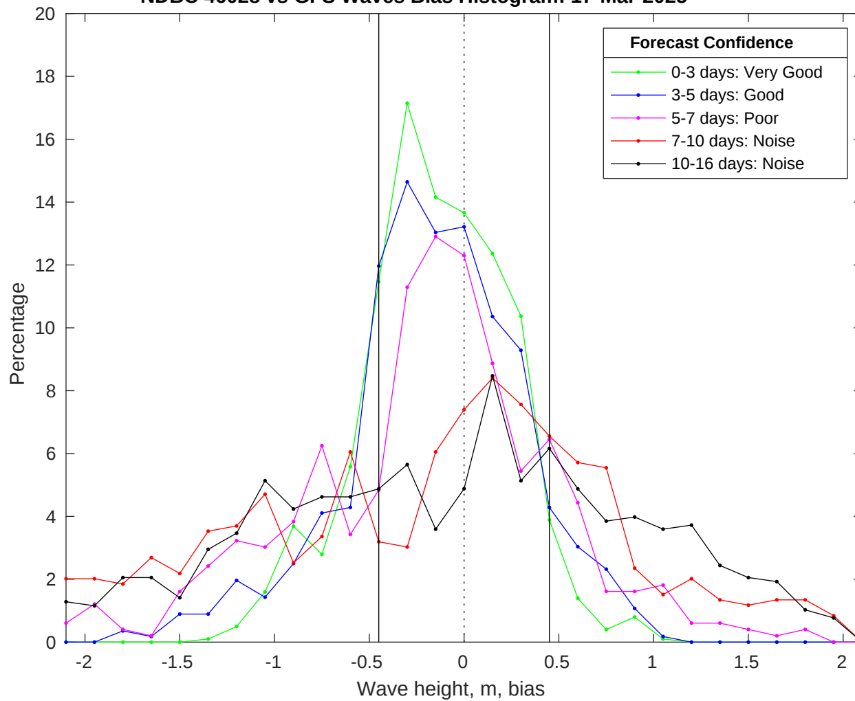
NDBC 46028 vs GFS Waves Bias Histogram: 17-Mar-2025
