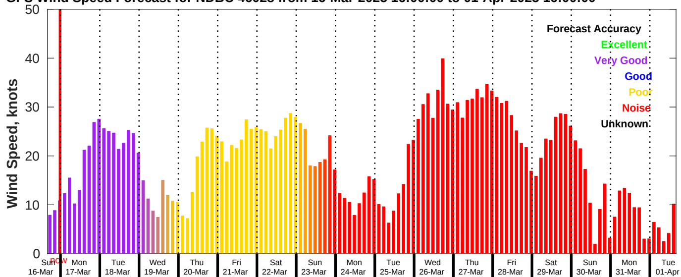
GFS Wind Speed Forecast for NDBC 46028 from 16-Mar-2025 16:00:00 to 01-Apr-2025 16:00:00
