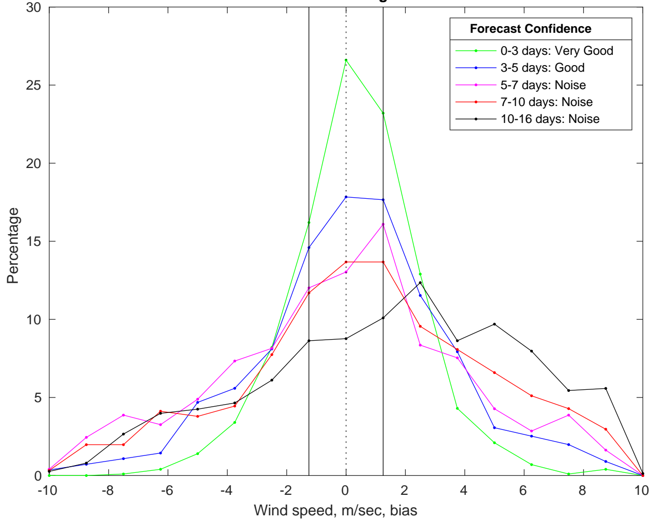
NDBC 46054 vs GFS Winds Bias Histogram: 17-Mar-2025
