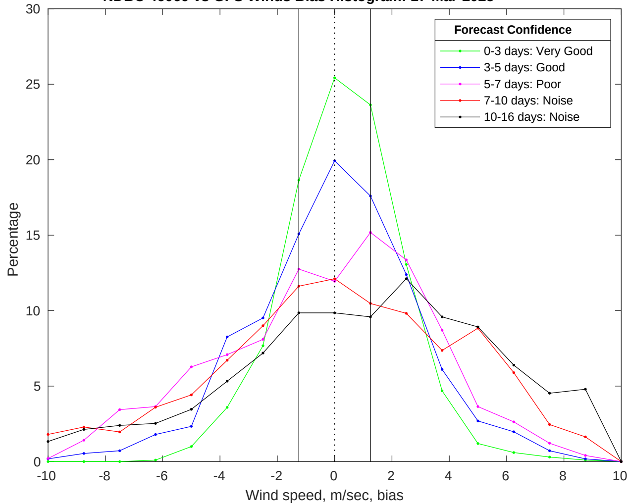
NDBC 46069 vs GFS Winds Bias Histogram: 17-Mar-2025
