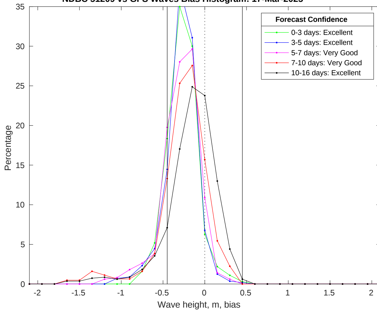
NDBC 51209 vs GFS Waves Bias Histogram: 17-Mar-2025
