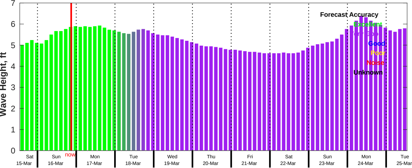
CMEMS Wave Forecast for NDBC 51209 from 15-Mar-2025 13:00:00 to 25-Mar-2025 13:00:00
