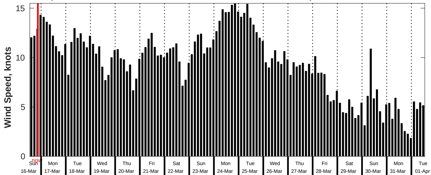
GFS Wind Speed Forecast for NDBC 51209 from 16-Mar-2025 13:00:00 to 01-Apr-2025 13:00:00
