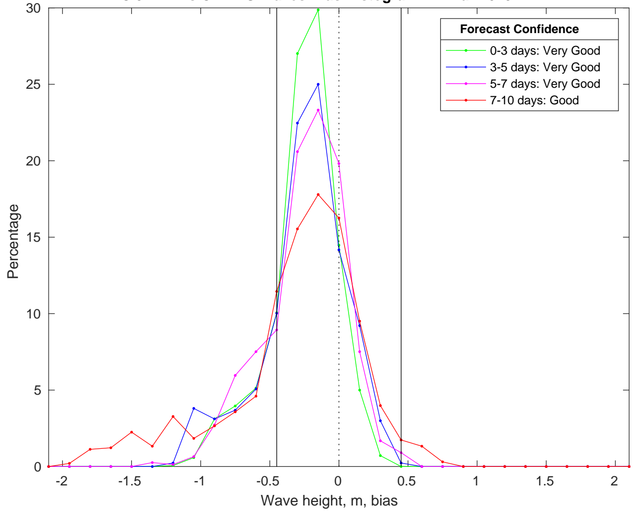
NDBC 52211 vs CMEMS Waves Bias Histogram: 17-Mar-2025
