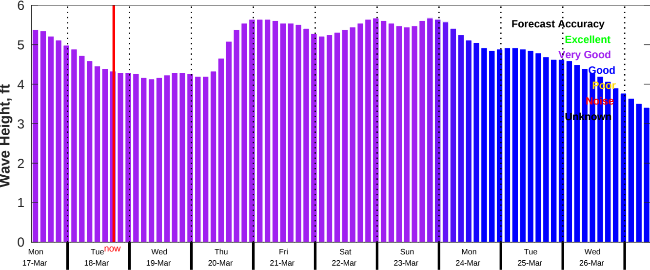
CMEMS Wave Forecast for NDBC 52211 from 16-Mar-2025 10:00:00 to 26-Mar-2025 10:00:00
