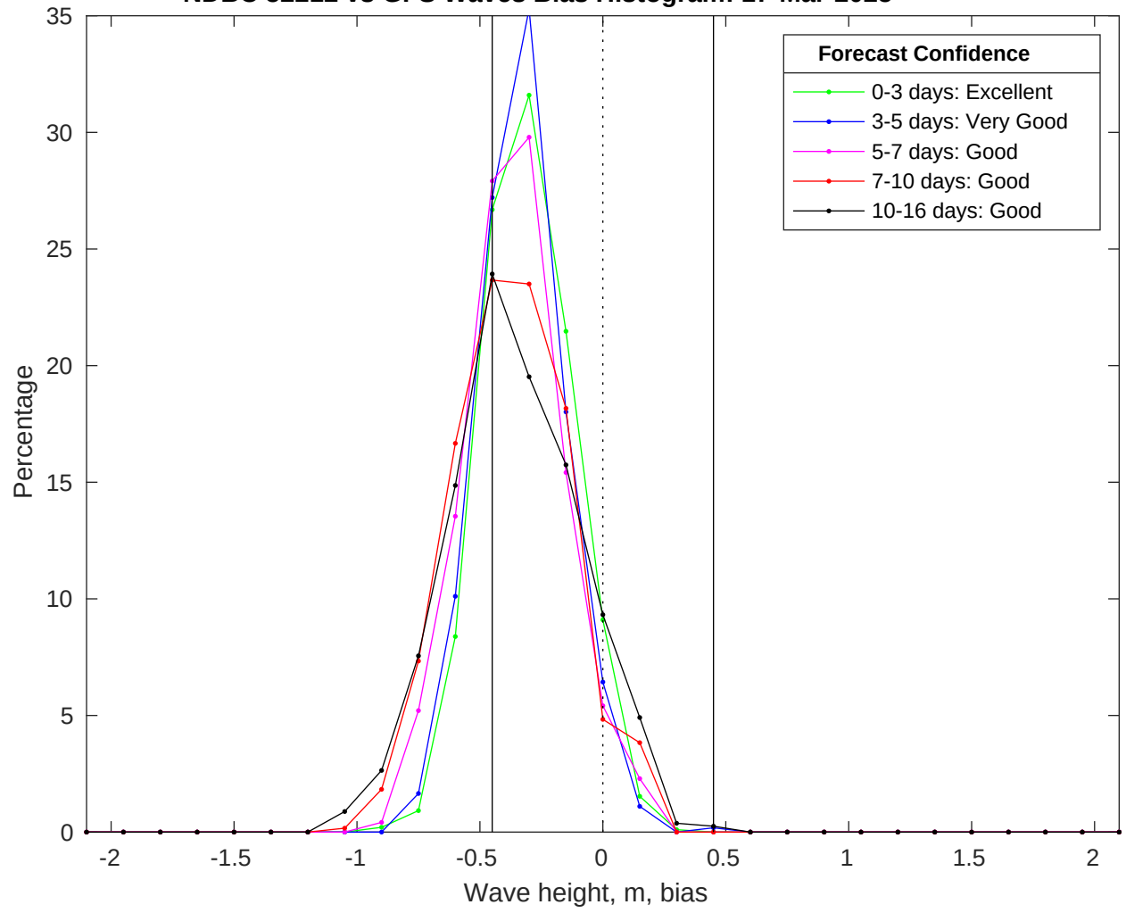
NDBC 52212 vs GFS Waves Bias Histogram: 17-Mar-2025
