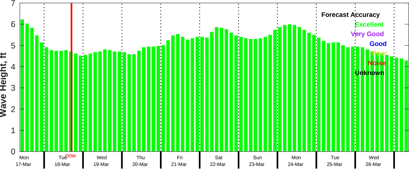
CMEMS Wave Forecast for NDBC 52212 from 16-Mar-2025 09:00:00 to 26-Mar-2025 09:00:00
