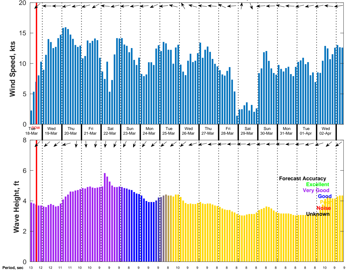
Wind & Wave Forecast for NDBC 52212 from 17-Mar-2025 09:00:00 to 02-Apr-2025 09:00:00
