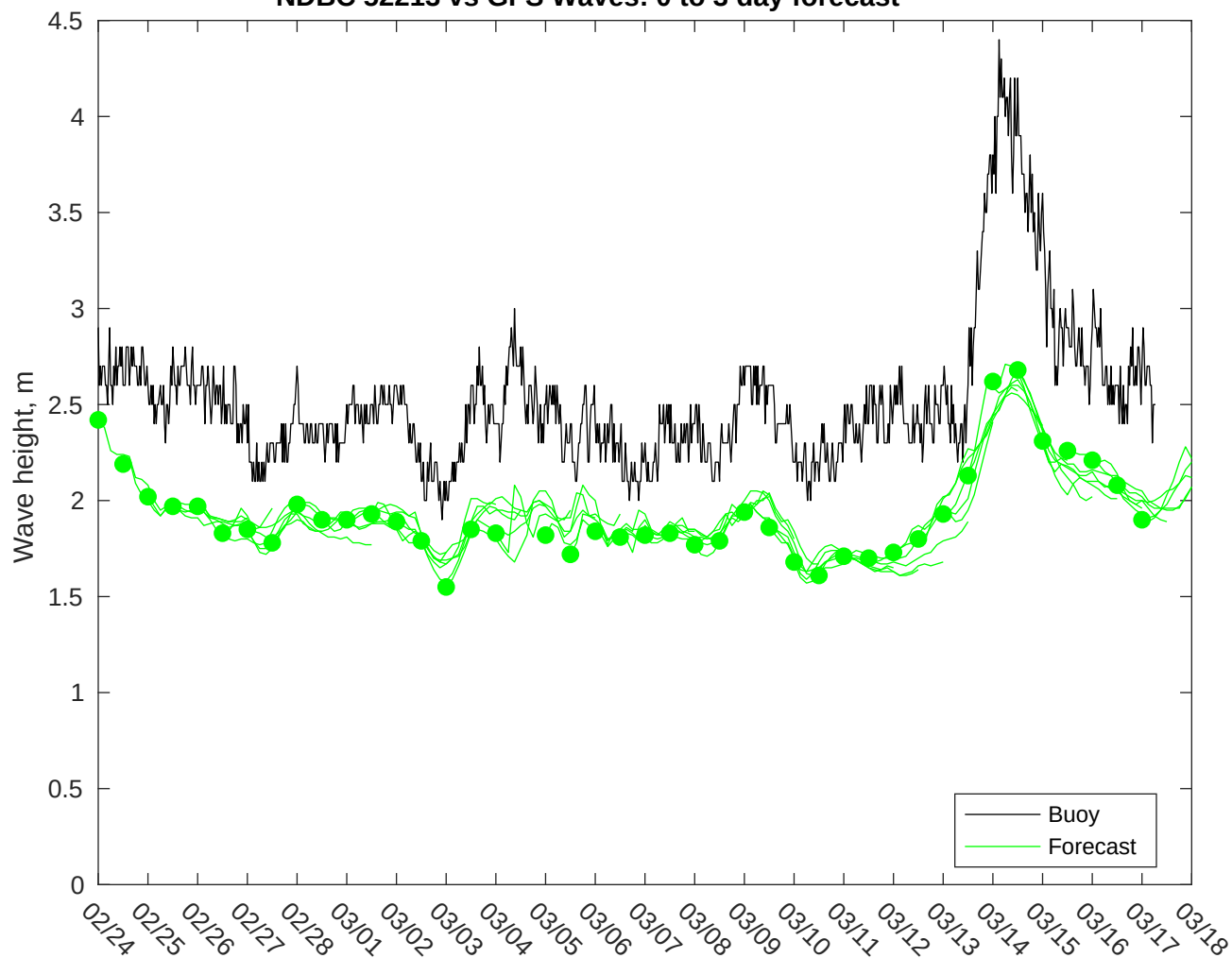
NDBC 52213 vs GFS Waves: 0 to 3 day forecast
