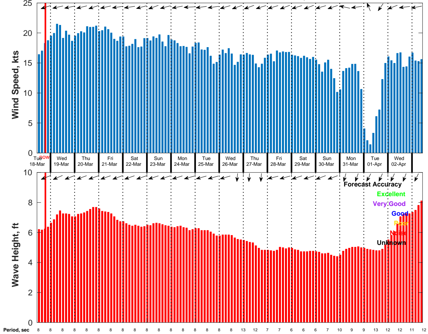
Wind & Wave Forecast for NDBC 52213 from 17-Mar-2025 11:00:00 to 02-Apr-2025 11:00:00
