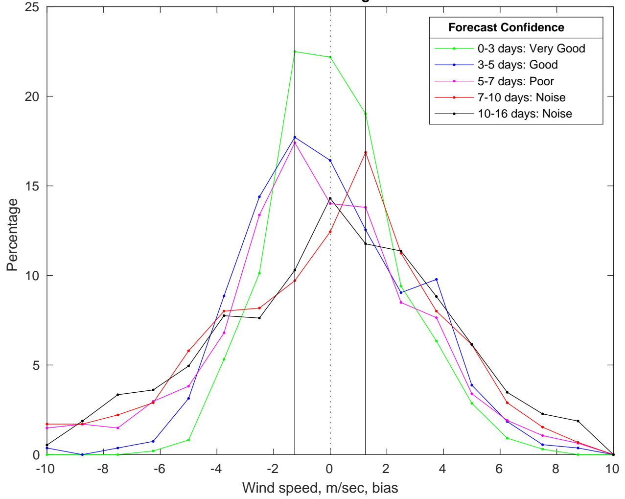
NDBC 41004 vs GFS Winds Bias Histogram: 18-Mar-2025
