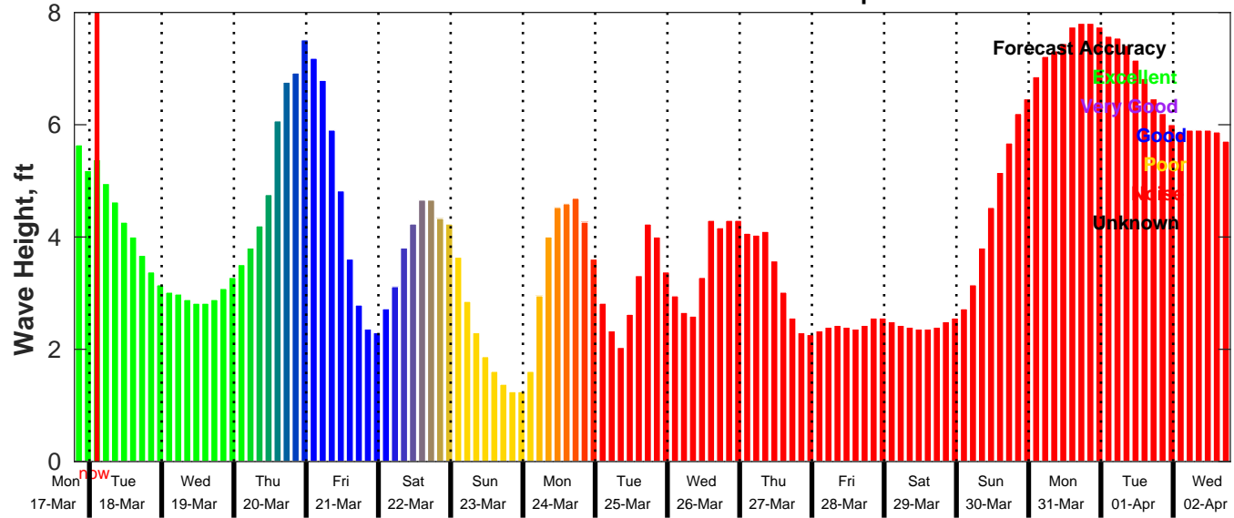
GFS Wave Forecast for NDBC 41004 from 17-Mar-2025 19:00:00 to 02-Apr-2025 19:00:00
