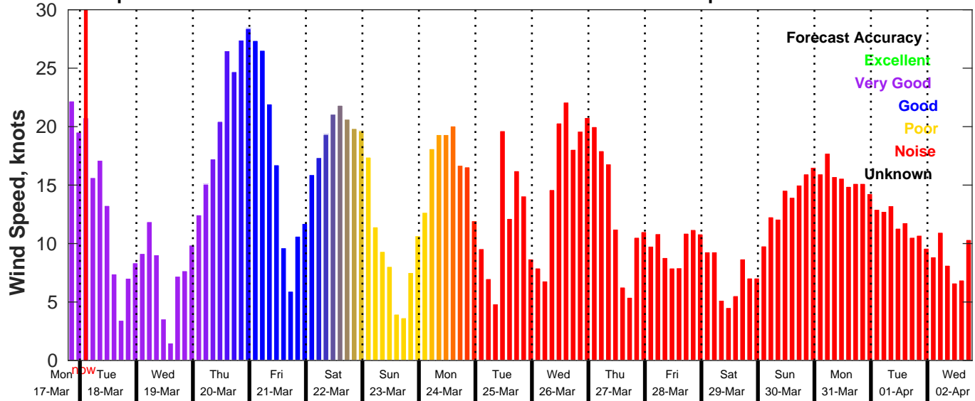
GFS Wind Speed Forecast for NDBC 41004 from 17-Mar-2025 19:00:00 to 02-Apr-2025 19:00:00
