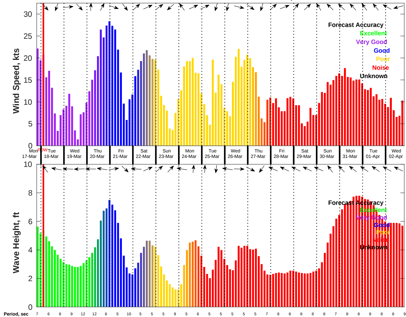
Wind & Wave Forecast for NDBC 41004 from 17-Mar-2025 19:00:00 to 02-Apr-2025 19:00:00
