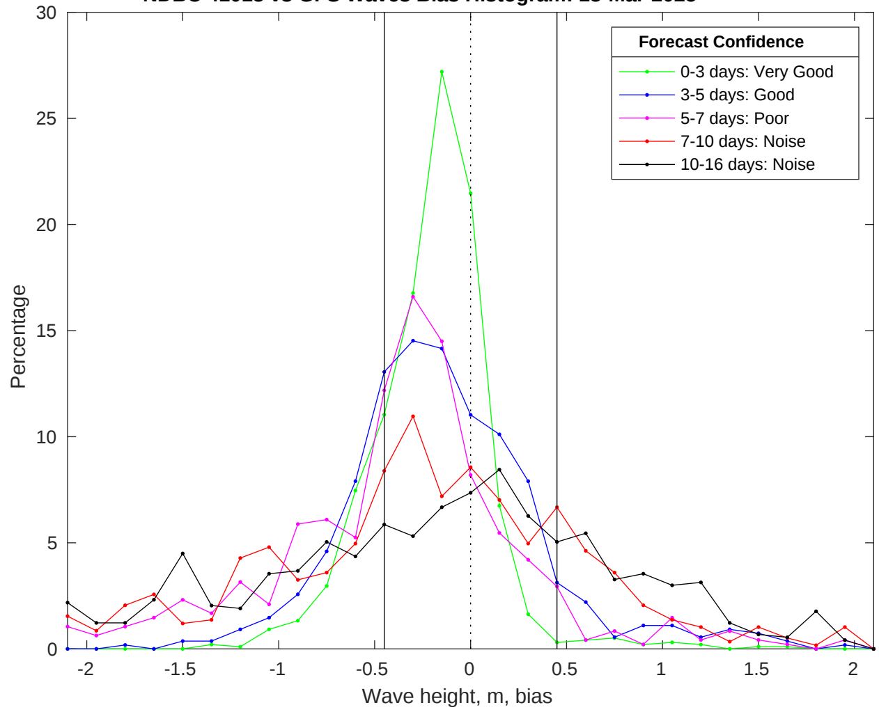
NDBC 41013 vs GFS Waves Bias Histogram: 18-Mar-2025
