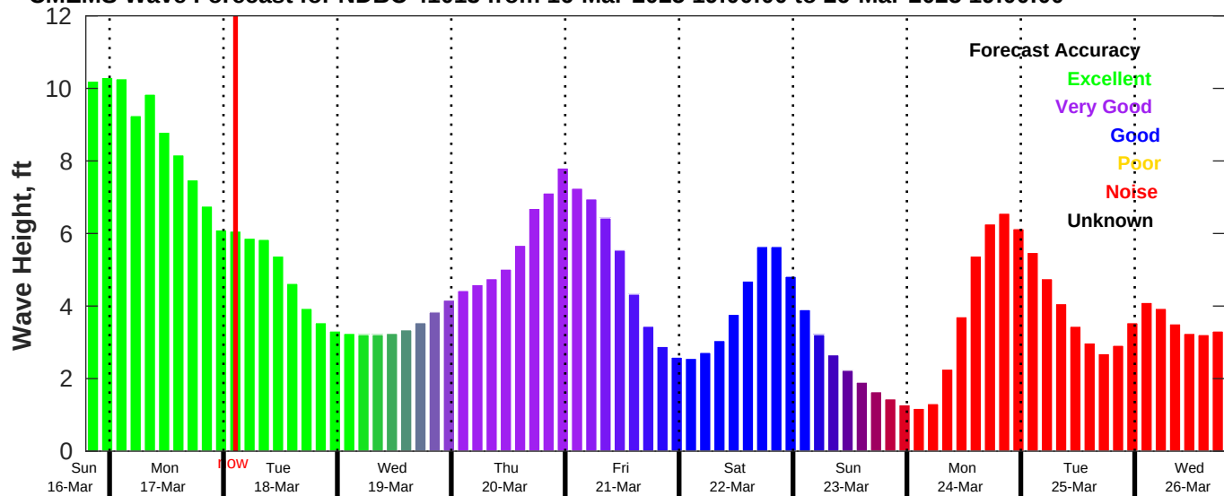
CMEMS Wave Forecast for NDBC 41013 from 16-Mar-2025 19:00:00 to 26-Mar-2025 19:00:00
