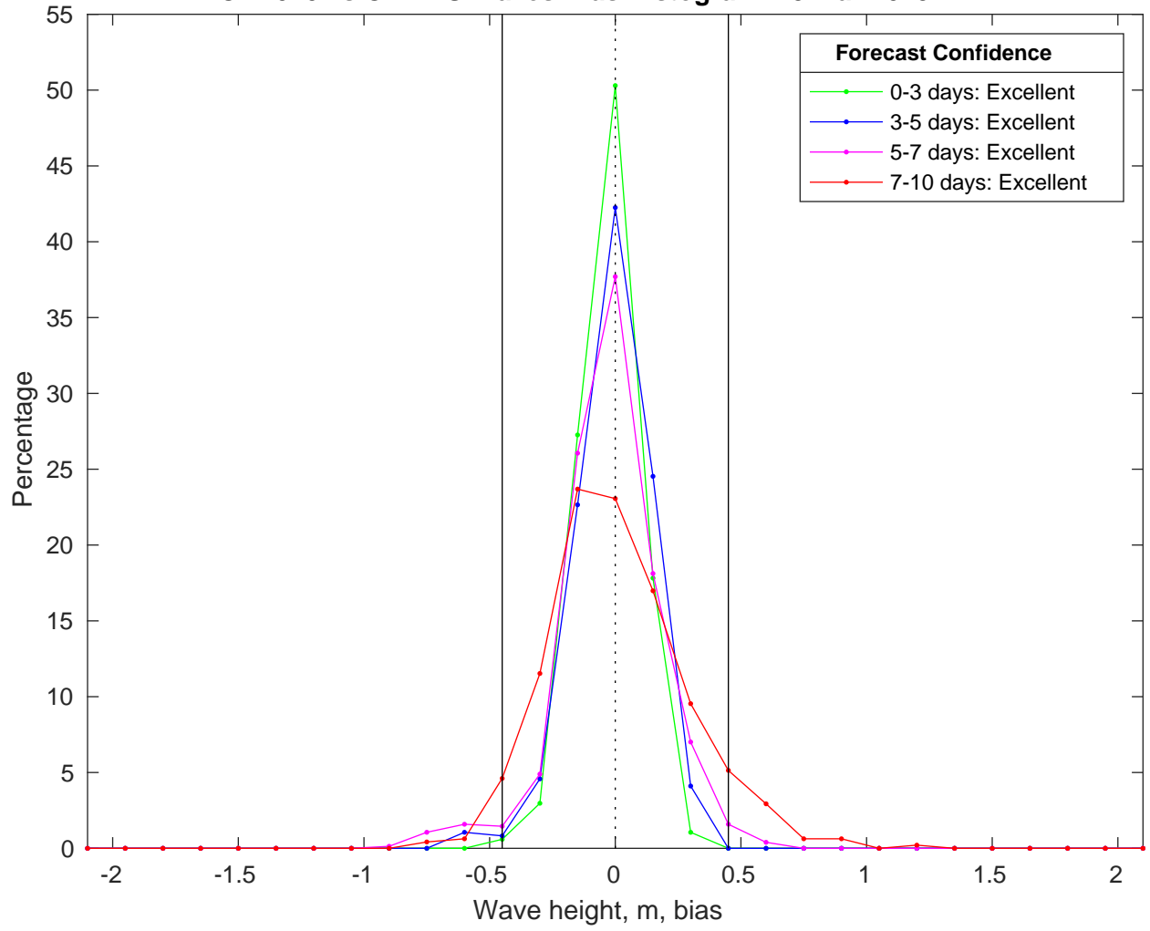
NDBC 41040 vs CMEMS Waves Bias Histogram: 18-Mar-2025
