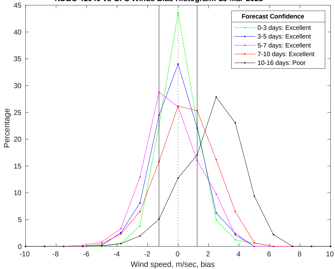
NDBC 41040 vs GFS Winds Bias Histogram: 18-Mar-2025
