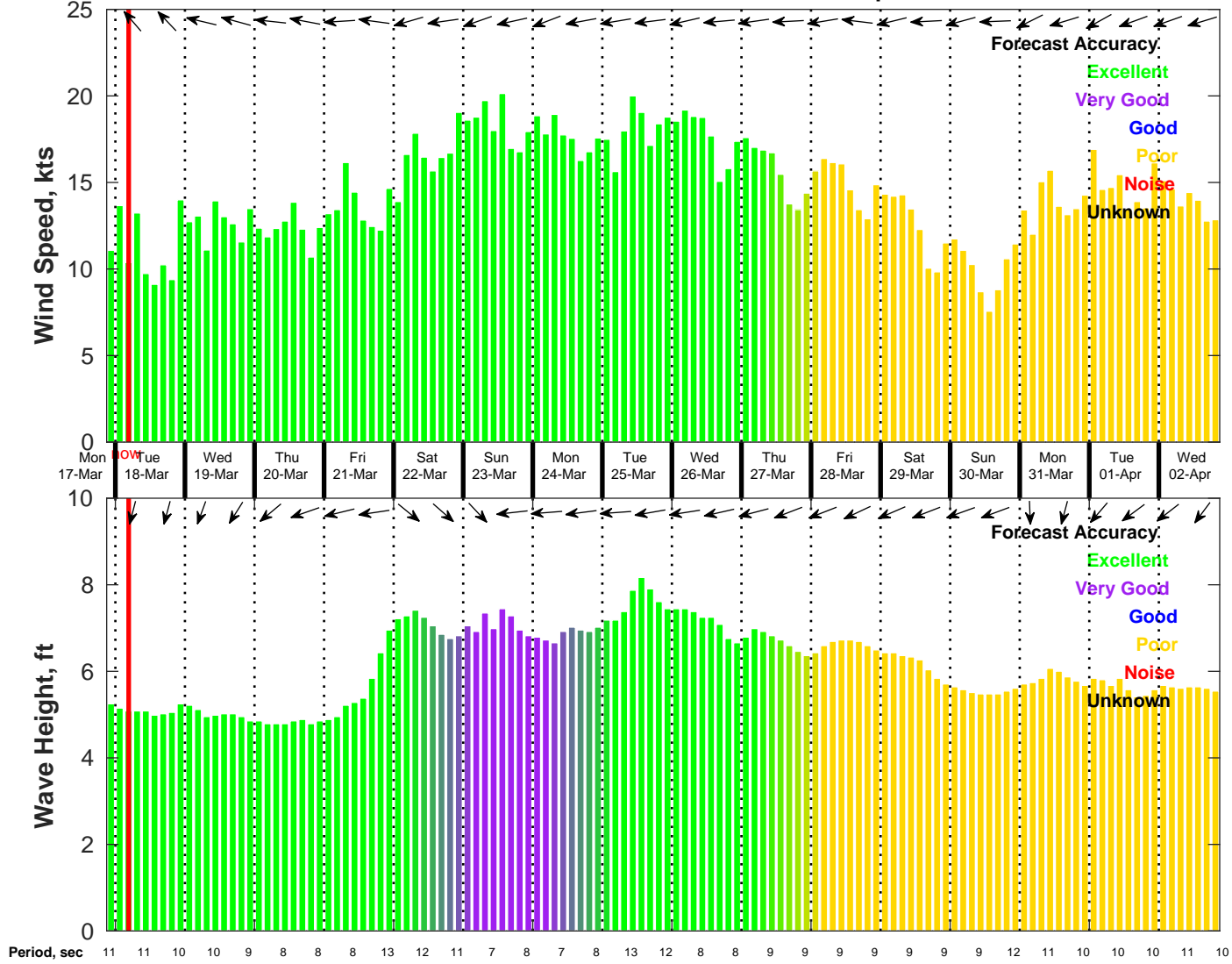
Wind & Wave Forecast for NDBC 41040 from 17-Mar-2025 21:00:00 to 02-Apr-2025 21:00:00
