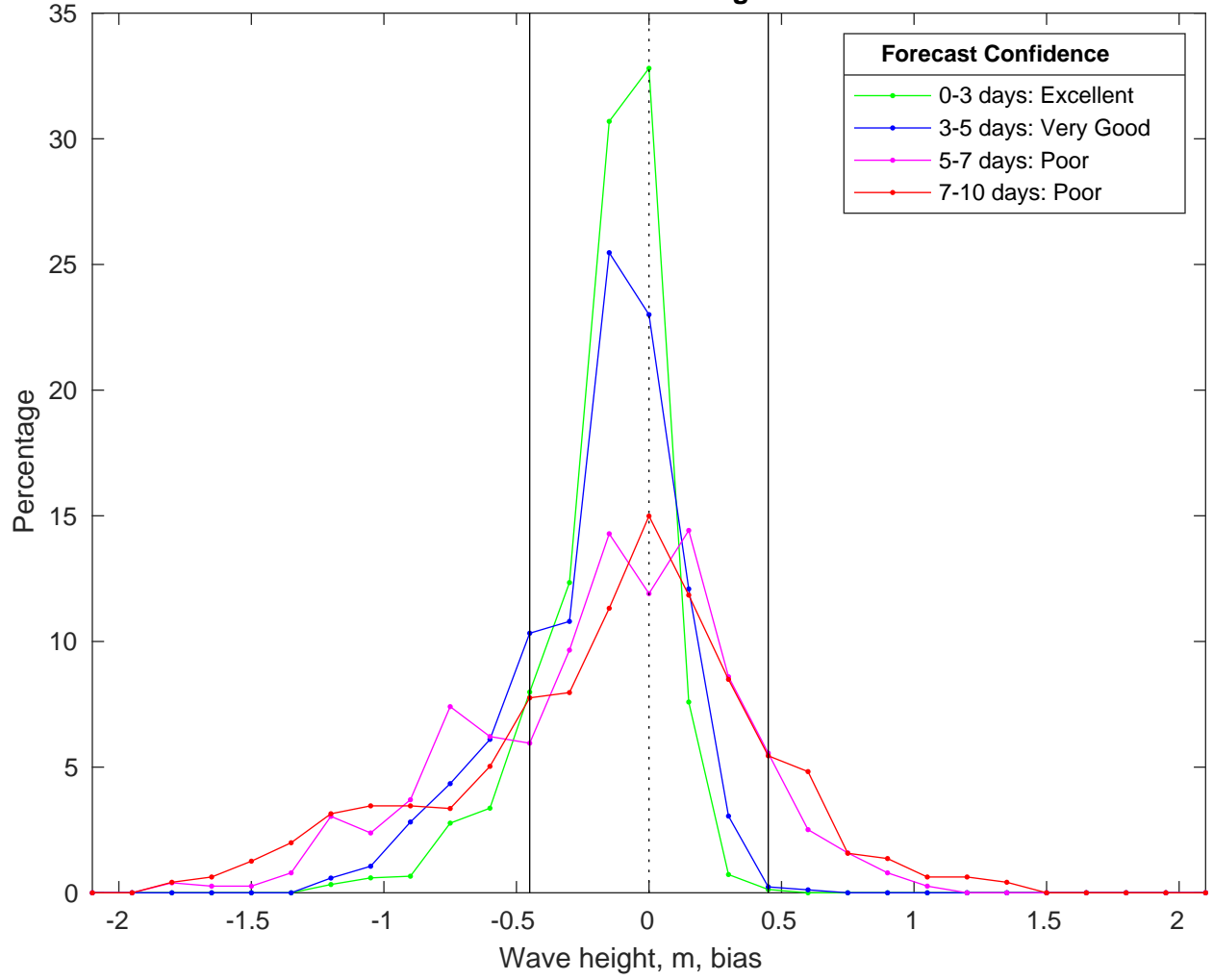
NDBC 42019 vs CMEMS Waves Bias Histogram: 18-Mar-2025
