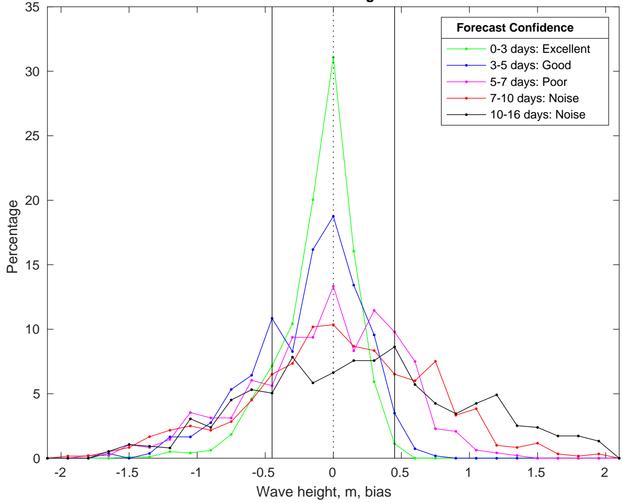
NDBC 42019 vs GFS Waves Bias Histogram: 18-Mar-2025
