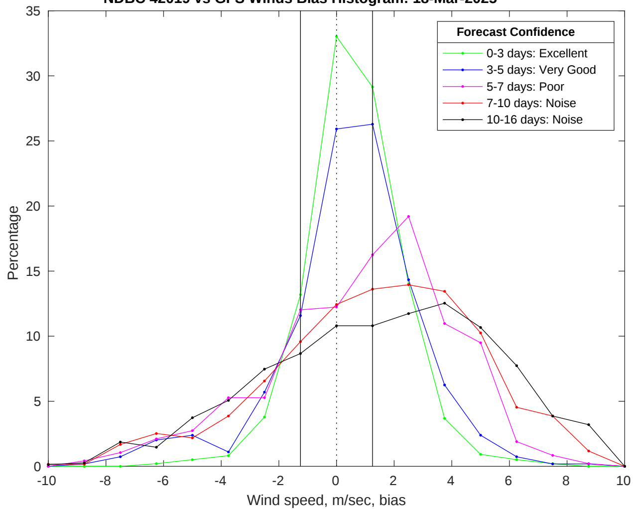
NDBC 42019 vs GFS Winds Bias Histogram: 18-Mar-2025
