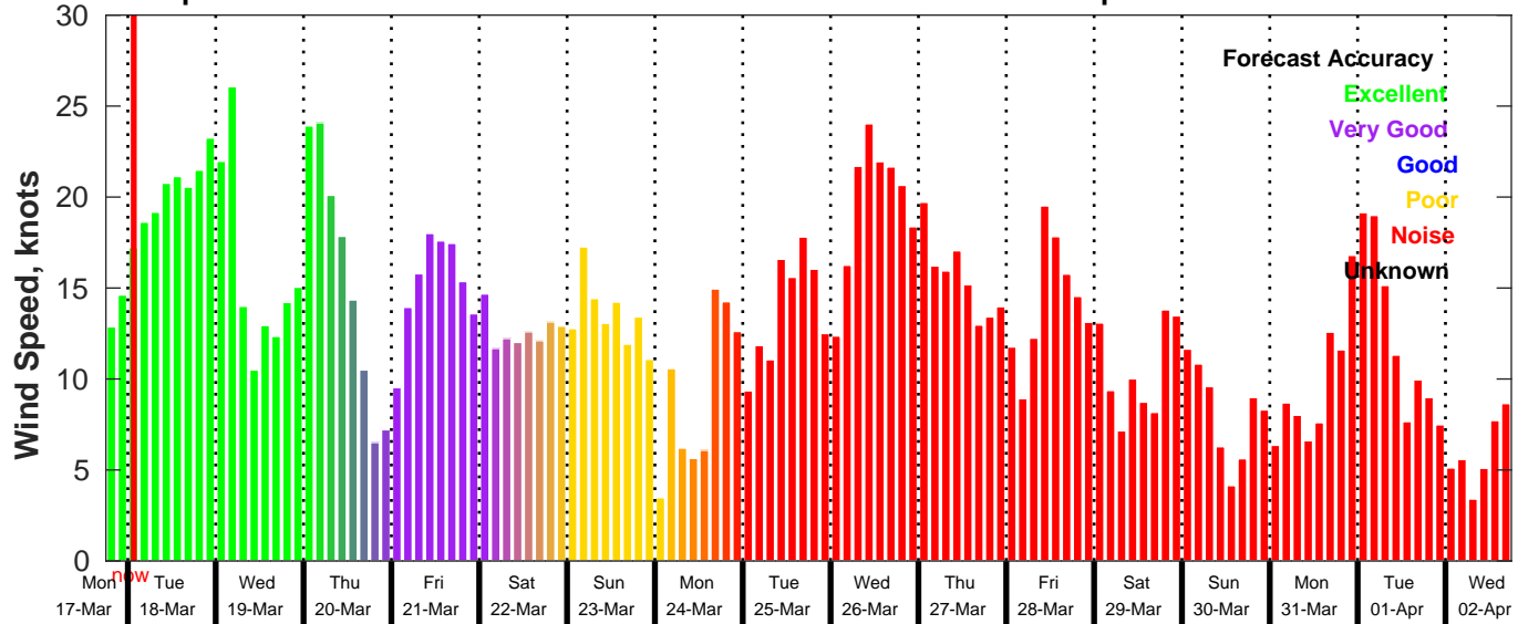
GFS Wind Speed Forecast for NDBC 42019 from 17-Mar-2025 18:00:00 to 02-Apr-2025 18:00:00
