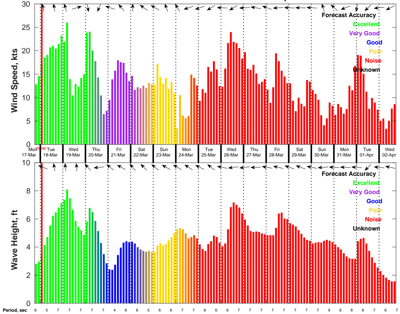
Wind & Wave Forecast for NDBC 42019 from 17-Mar-2025 18:00:00 to 02-Apr-2025 18:00:00
