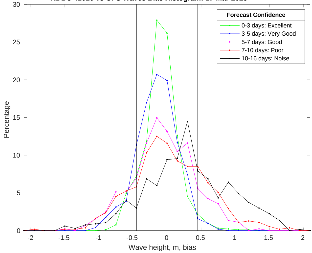
NDBC 42020 vs GFS Waves Bias Histogram: 17-Mar-2025
