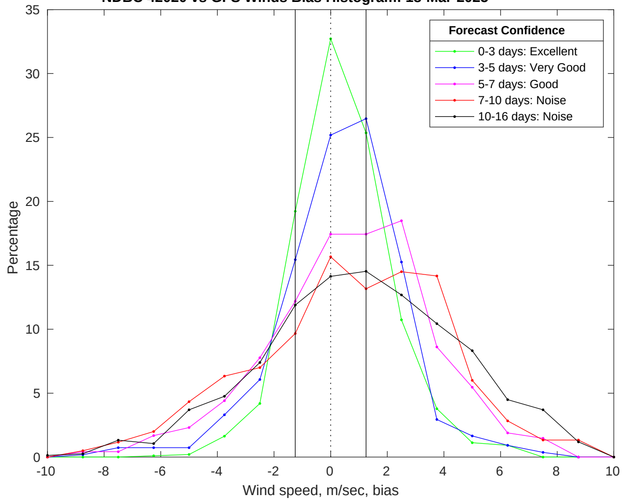
NDBC 42020 vs GFS Winds Bias Histogram: 18-Mar-2025
