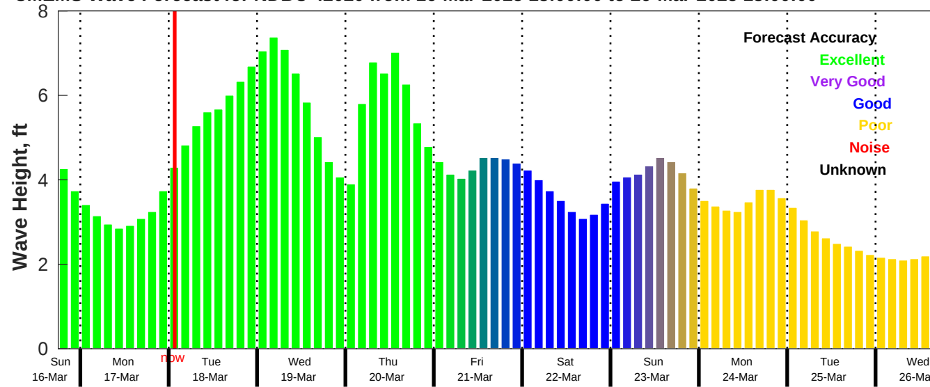
CMEMS Wave Forecast for NDBC 42020 from 16-Mar-2025 18:00:00 to 26-Mar-2025 18:00:00
