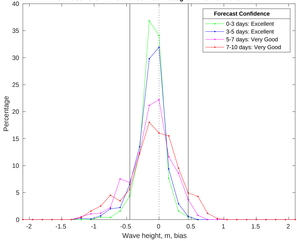
NDBC 42035 vs CMEMS Waves Bias Histogram: 18-Mar-2025
